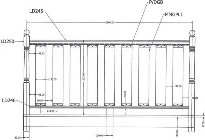
Plate 3: Drawing of Softwood Decking Glass Panel System
