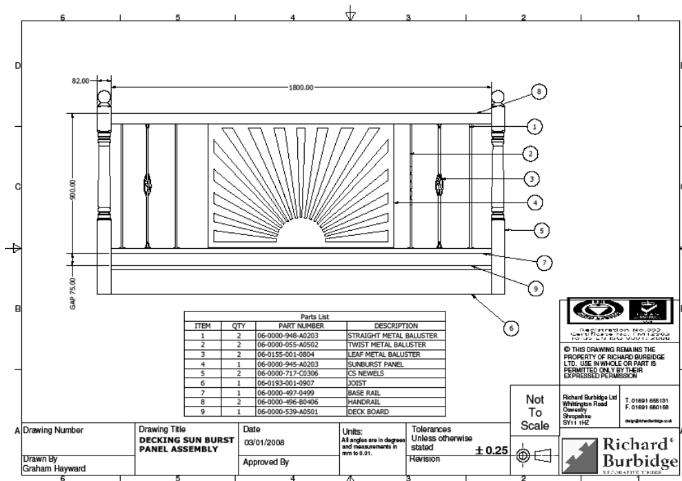
Plate 2: Technical Drawing
